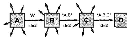
Fig. 1. Example of DSR Route Discovery
